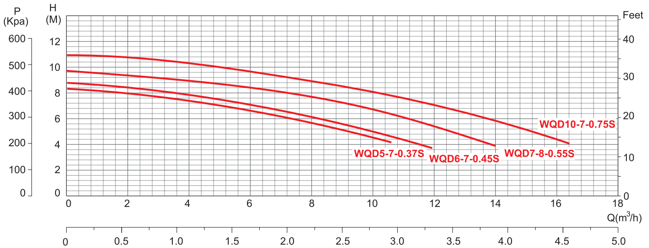
Performance table (n=2900r/min)
